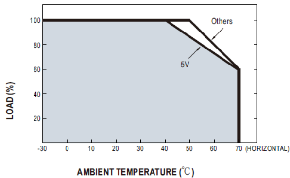
■ Derating Curve
